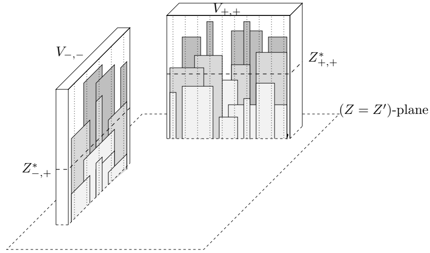
Figure 7: The darker vertices are hidden on all levels between Z' and Z_{-,+}^* ( Z_{+,+}^* ), whereas the lighter vertices are inactive on all levels z \geq Z_{-,+}^* ( z \geq Z_{+,+}^* ). (Only the projection of the vertices onto the bounding box is shown. Also, the picture is simplified in that only one of two possible directions of exposure is considered.)
