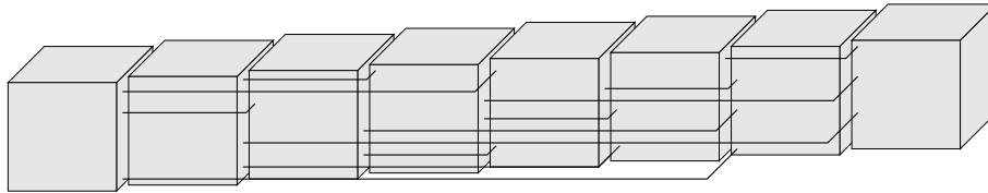
Figure 2: A cube-drawing of K_n with volume O(n^4) . Only half of the edges are shown; the other half is routed behind the cubes.
