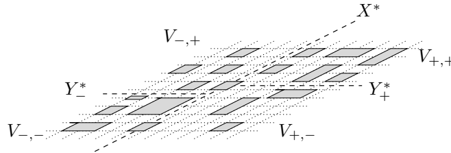
Figure 5: Illustration of case (2).
