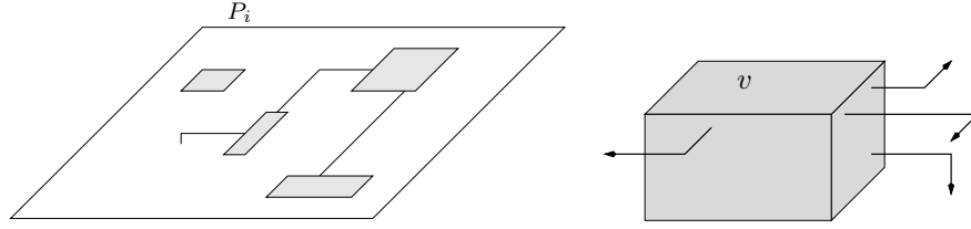
Figure 1: Illustration of n(P_i) and p(v) . In the left picture n(P_i) = 3 , because while four vertices intersect P_i , only three of them are incident to an edge that belongs to P_i . In the right picture, p(v) = 2 .
