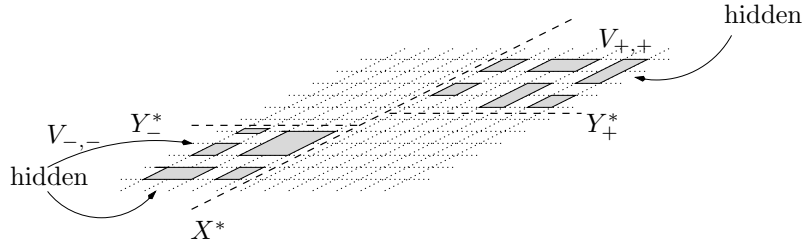
Figure 6: Examples of hidden vertices (we only show the cross-section with one Z -plane). All vertices not marked otherwise are exposed. Note that the top right vertex is hidden even though there is an X -line from it not intersecting other vertices, because this X -line is not a grid-line.
