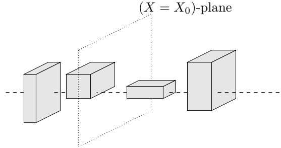
Figure 4: Illustration of case (1).
