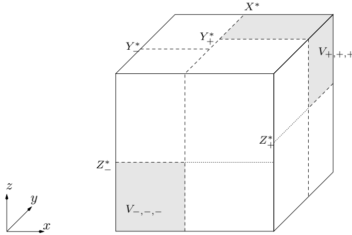
Figure 3: Two diagonally opposite octants yield two non-empty sets of vertices that cannot have an edge with 0 or 1 bends connecting them.
